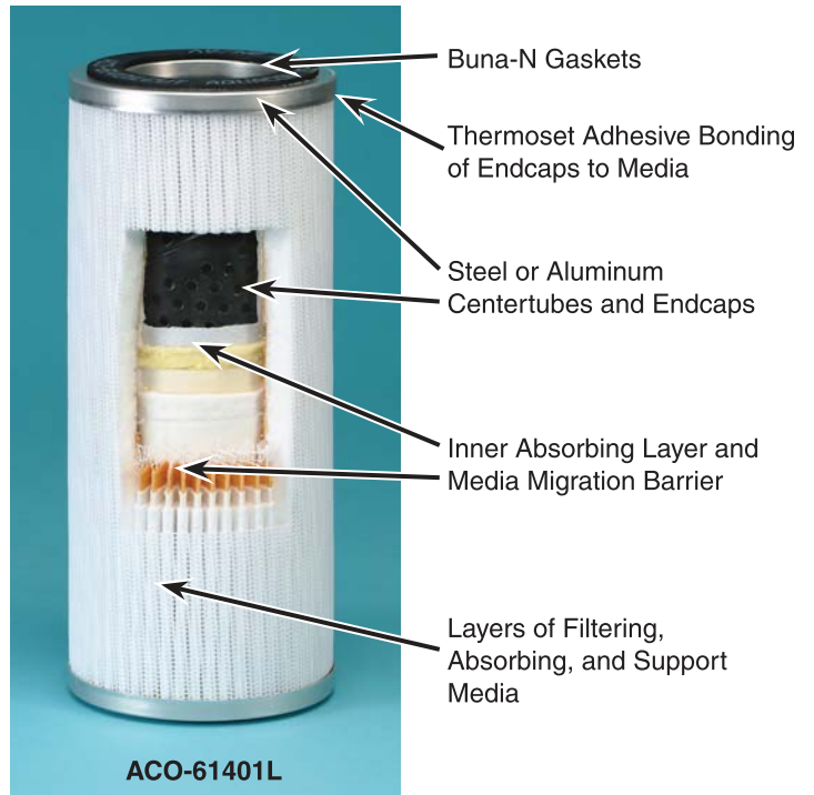
Typical Aquacon Cartridge Construction
